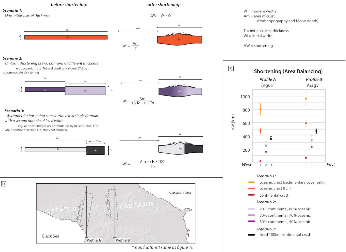
Figure 4 – a) Model and input parameters for area balancing. b) Locations of area balancing profiles. Profile A roughly aligns with the Enguri cross section (Figure 2), while Profile B roughly aligns with the Aragvi cross section (Figure 3). c) Results of area balancing exercise for the western Greater Caucasus orogen.
